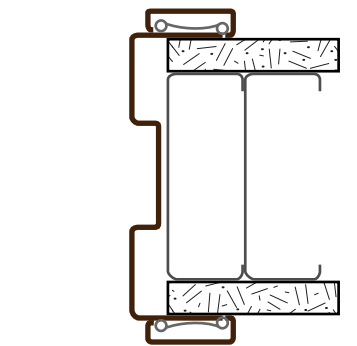
6V Jamb - Inverted Stop
